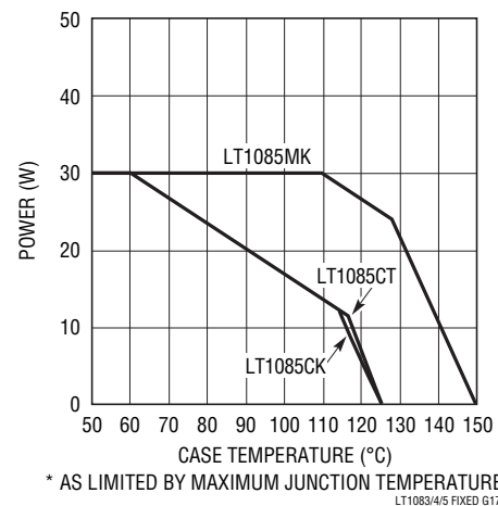
LT1085 Maximum Power Dissipation*
