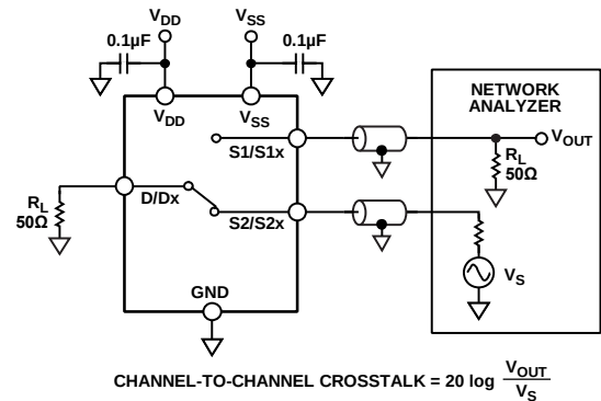
Figure 42. Channel-to-Channel Crosstalk
