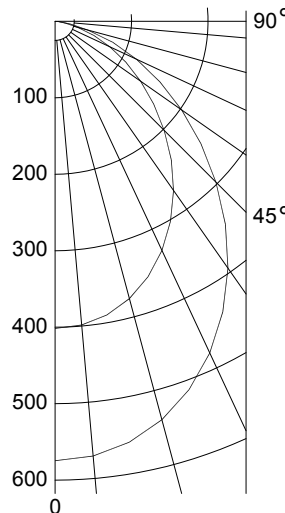
Zonal Lumens - 850
