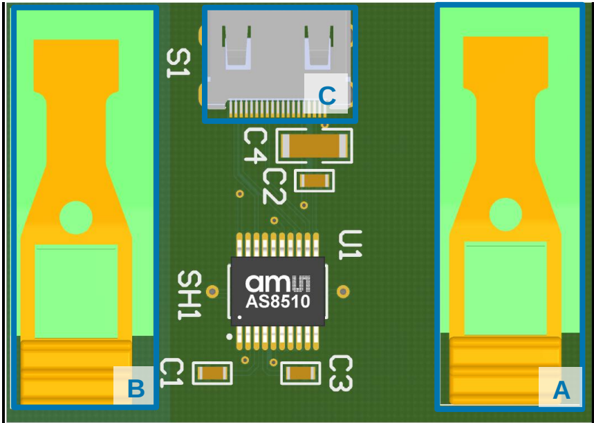
Figure 2: PCB Connection Diagram
