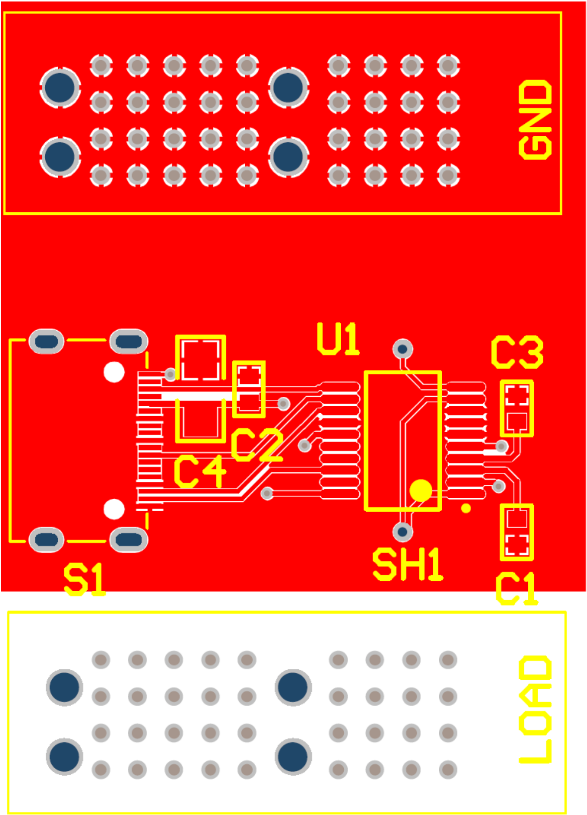
Figure 5: Top Layer
