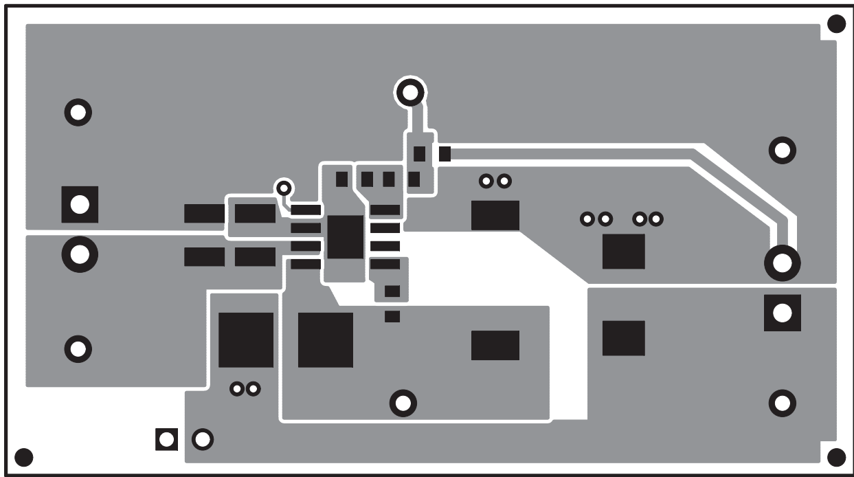
Figure 7. Top-side Layout
