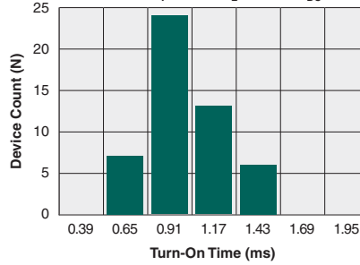
Typical Turn-On Time (N=50, I F =5mA, I L =200mA DC )
