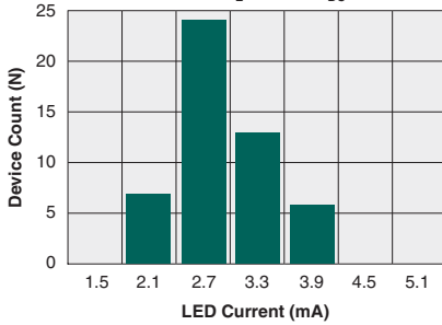
Typical I F for Switch Operation (N=50, I L =200mA DC )
