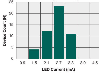
Typical I F for Switch Dropout (N=50, I L =200mA DC )
