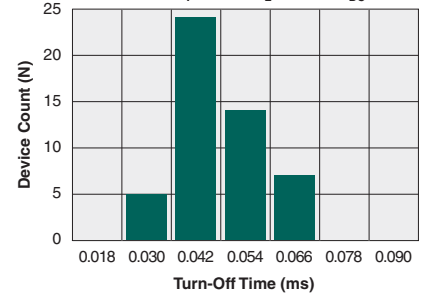
Typical Turn-Off Time (N=50, I F =5mA, I L =200mA DC )
