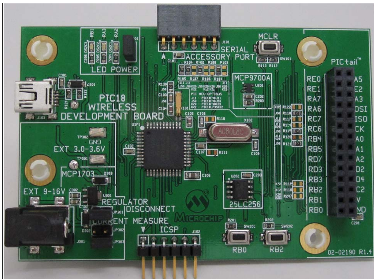
FIGURE 2-1: PIC18 WIRELESS DEVELOPMENT BOARD
