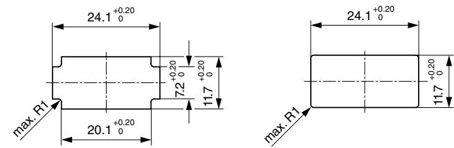
Panel cut-out for X = 1.0 mm
