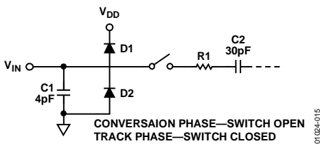
Figure 15. Equivalent Analog Input Circuit
