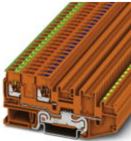
Sensor/actuator terminal block, Connection method: Push-in connection, Cross section: 0.2 mm 2 - 4 mm 2 , AWG: 24 - 12, Width: 7 mm, Color: orange, Mounting type: NS 35/7,5, NS 35/15
