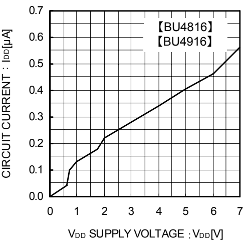
Fig.3 Circuit Current
