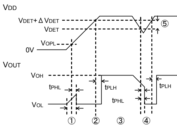
Fig. 14 Timing Waveforms
