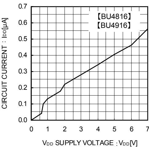
Fig.3 Circuit Current
