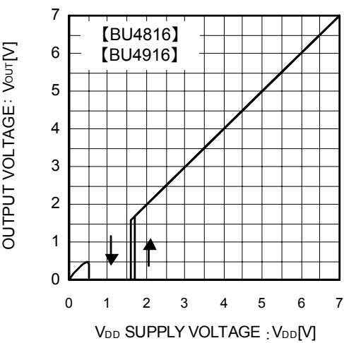
Fig.6 I/O Characteristics
