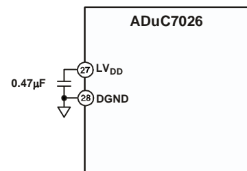
Figure 40: voltage regulator connections
