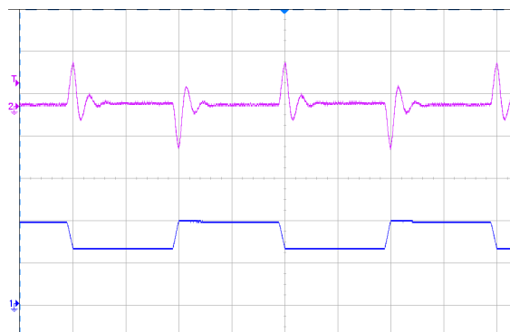
Figure 4 Dynamic response for 25% load step (50% ~ 75% ~ 50%) and 0.1A/ \mu s slew rate, (2ms/div), see Figure 10 for test configuration; CH2-output voltage (200mV/div); CH1-output current (10A/div)
