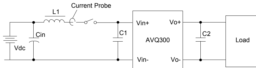
Figure 14 Input ripple & inrush current, ripple & noise test configuration
