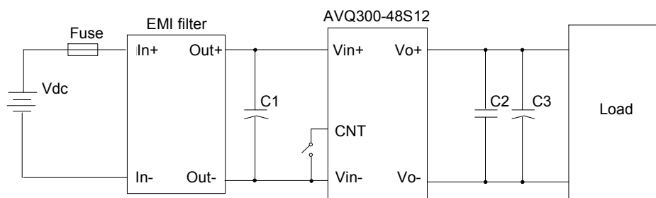
Figure 10 Typical application
