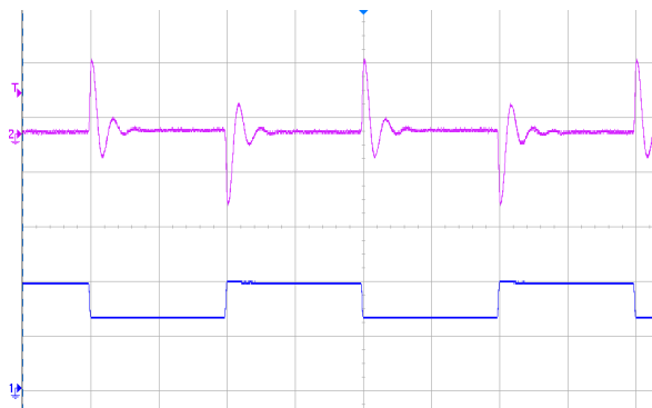
Figure 5 Dynamic response for 25% load step (50% ~ 75% ~ 50%) and 1A/ \mu s slew rate, (2ms/div), see Figure 10 for test configuration; CH2-output voltage (200mV/div); CH1-output current (10A/div)
