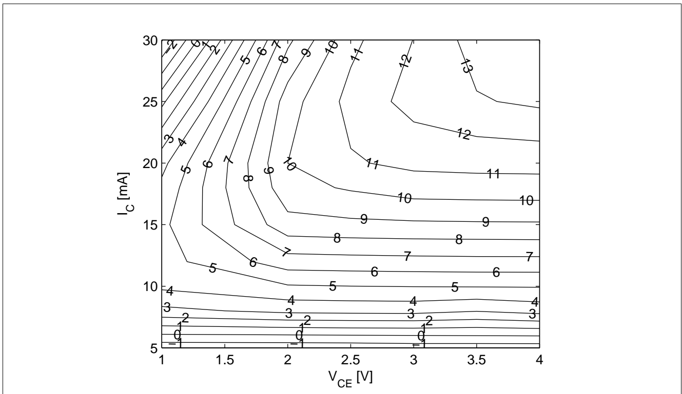
Figure 5-10 Compression Point at output OP_{1dB} [dBm] = f(I_C, V_{CE}) , Z_S = Z_L = 50 \Omega , f = 2.4 \text{ GHz}
