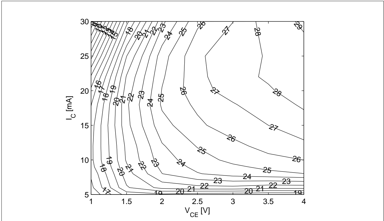
Figure 5-9 3rd Order Intercept Point at output OIP3 [dBm] = f(I_C, V_{CE}) , Z_S = Z_L = 50 \Omega , f = 2.4 \text{ GHz}
