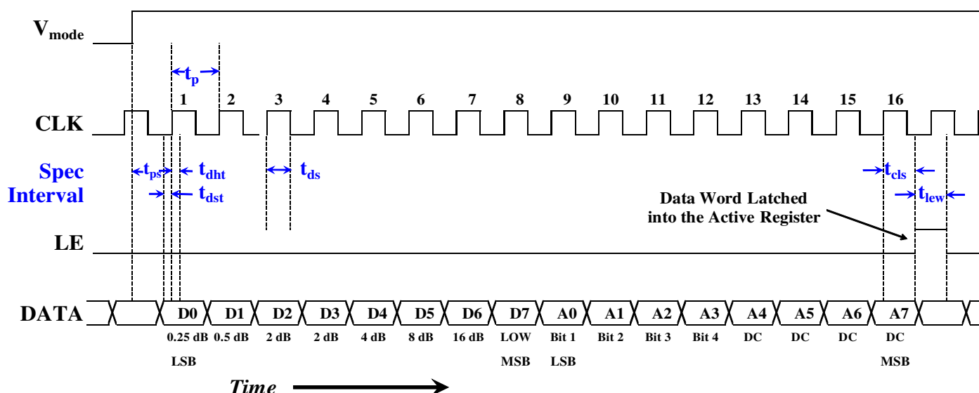
Figure 4 - Serial Timing Diagram
