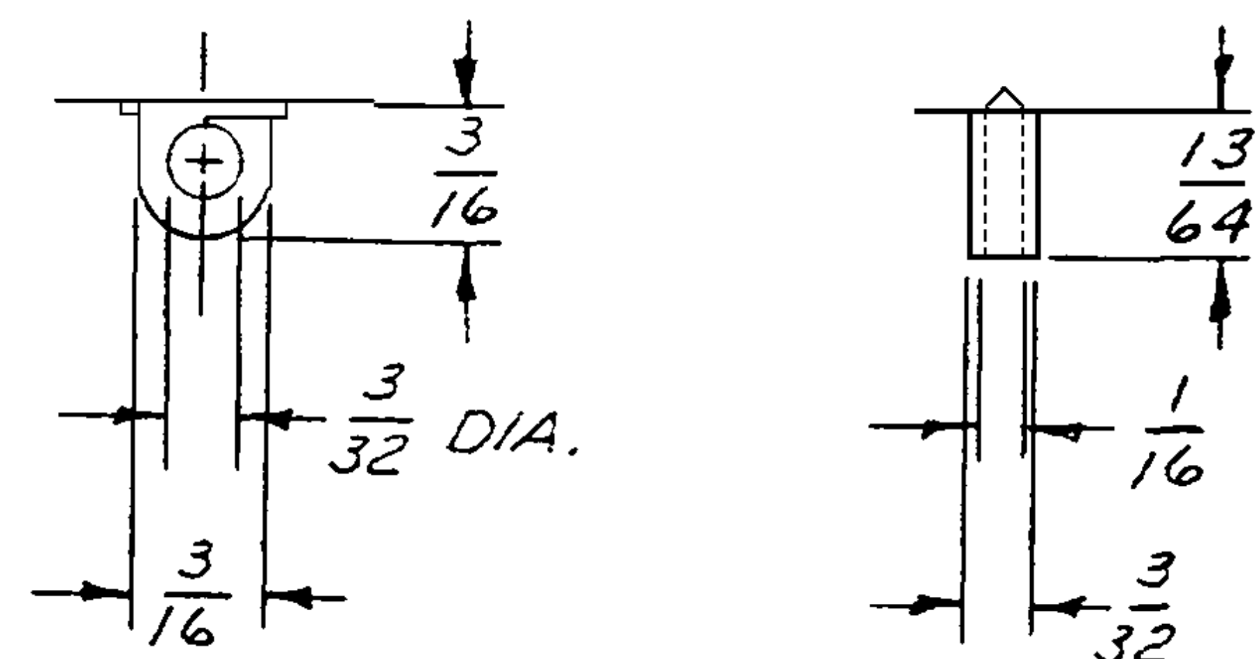
TERMINAL DETAIL
