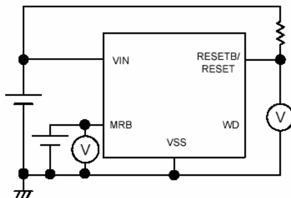
Circuit 9
