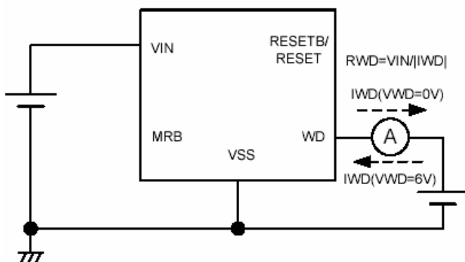
Circuit 8
