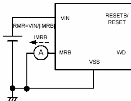
Circuit 11
