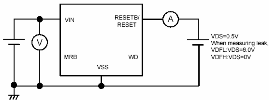
Circuit 4
