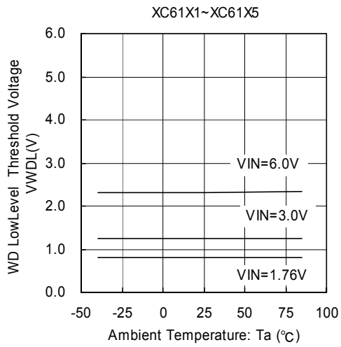
(12) Watchdog Low Level Voltage vs. Ambient Temperature
