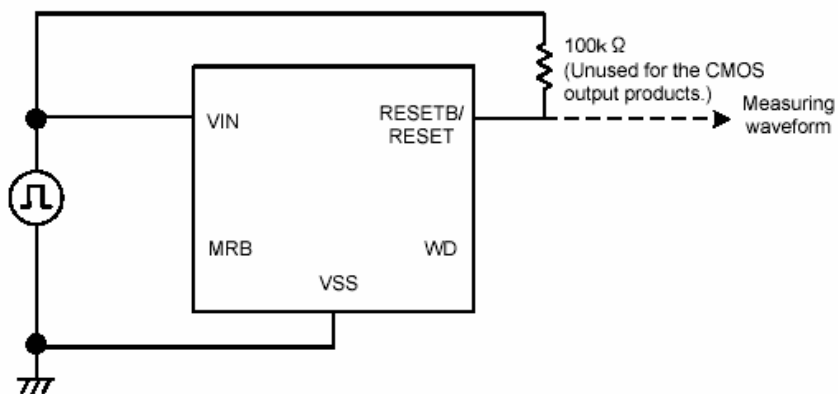
Circuit 7
