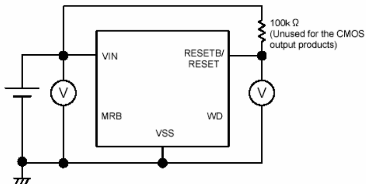
Circuit 1
