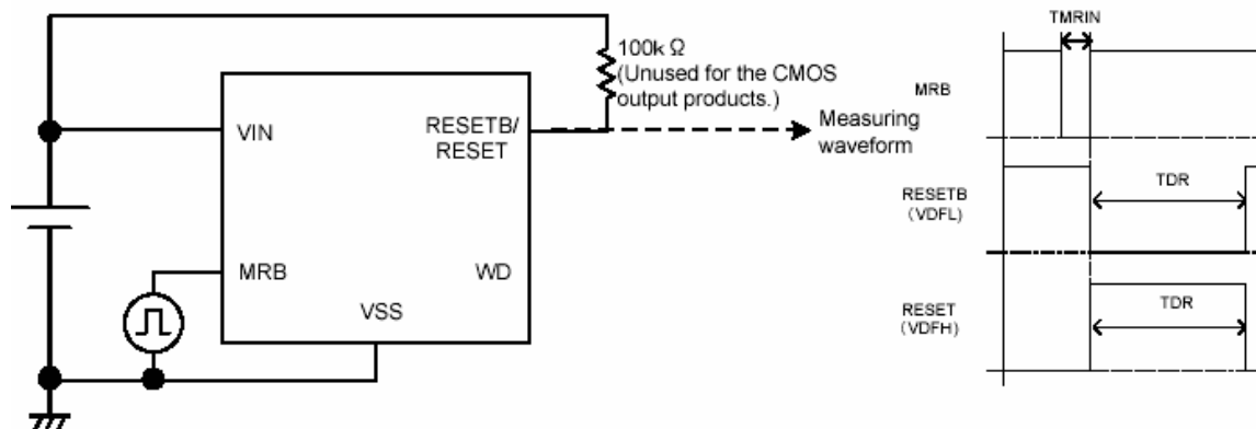
Circuit 11
