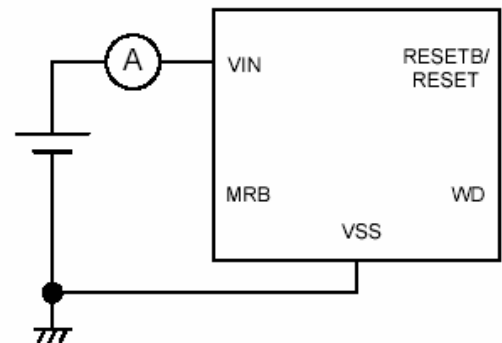
Circuit 2
