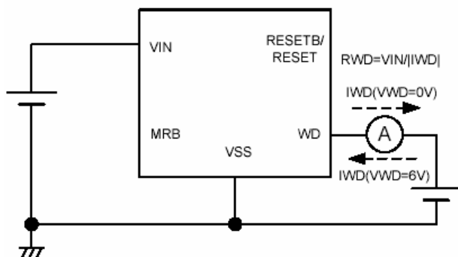
Circuit 8
