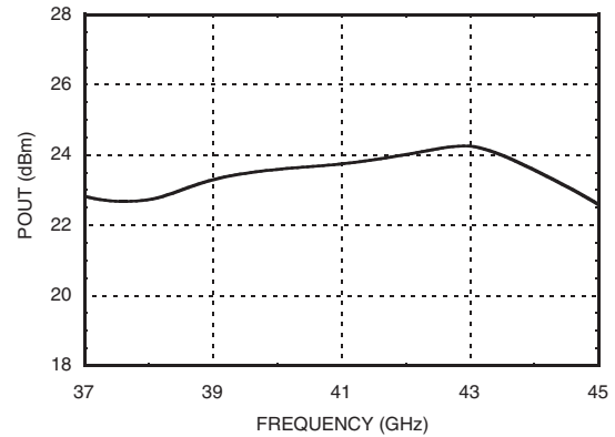
Fixtured P1dB vs. Frequency
