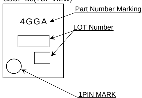
SSOP-B8(TOP VIEW)
