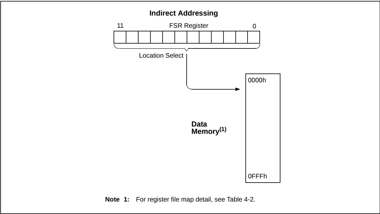
FIGURE 4-10: INDIRECT ADDRESSING
