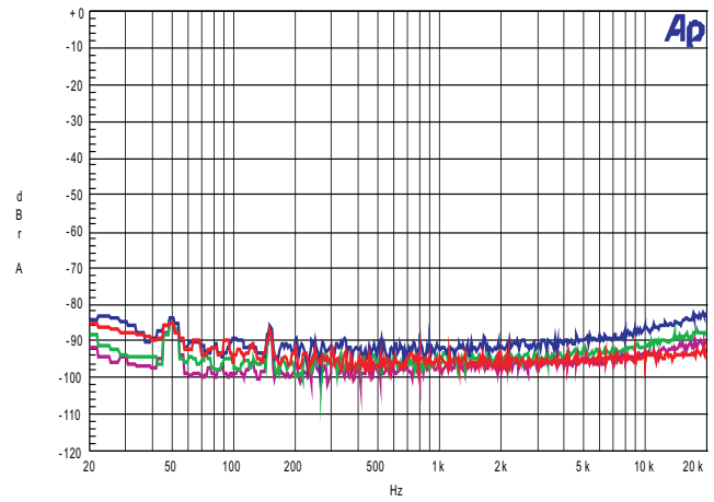
8. Noise Floor
