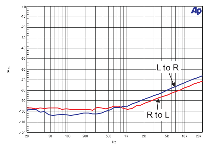
6. Crosstalk
