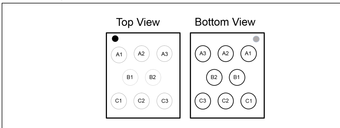
Figure 1c. W25Q10EW Ball Assignments, 8-ball WLCSP (Package Code BY)
