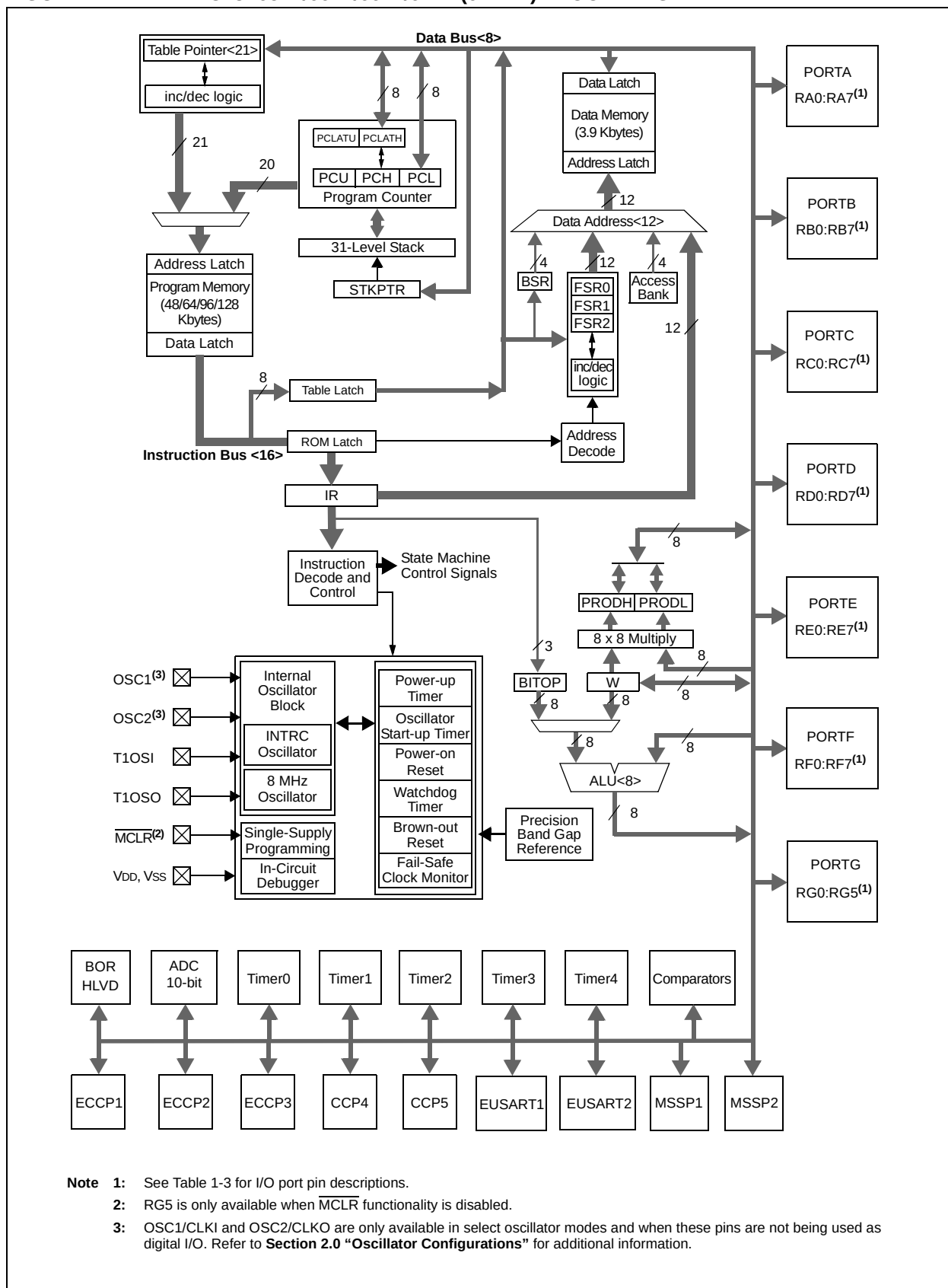
FIGURE 1-1: PIC18F6527/6622/6627/6722 (64-PIN) BLOCK DIAGRAM
