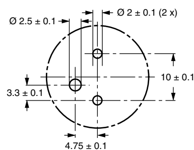
Fig.3 Mounting hole diagram
