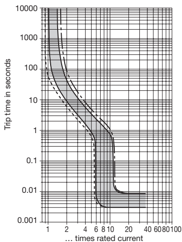
-T1 8...32 A
