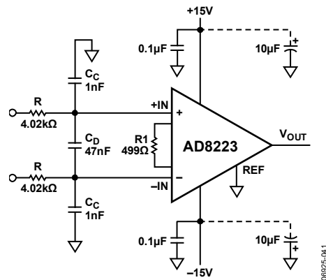
Figure 34. RFI Suppression
