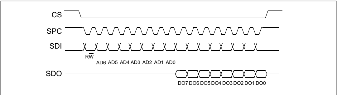
Figure 17. SPI read protocol
