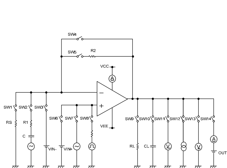
Figure 27. Test Circuit 2 (each Op-Amp)
