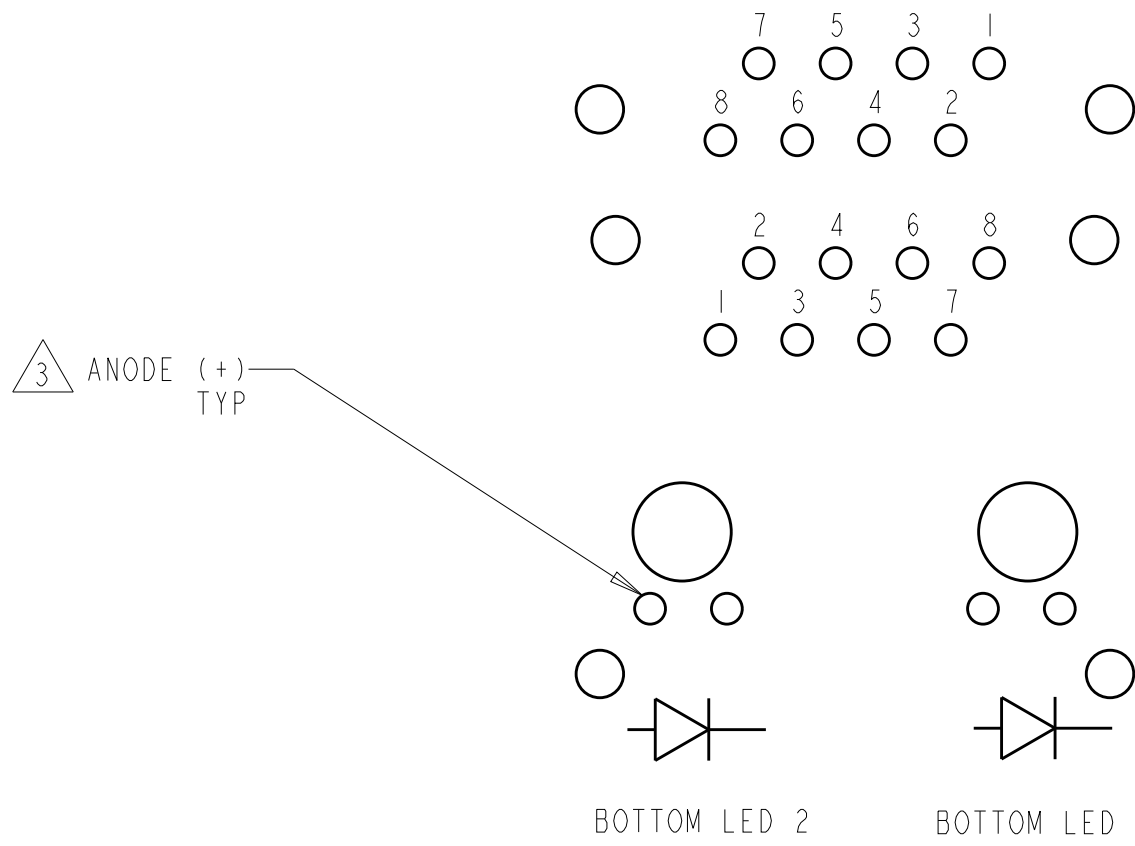
SCHEMATIC FOR 6368011-7, 1-6368011-2, 1-6368011-3
