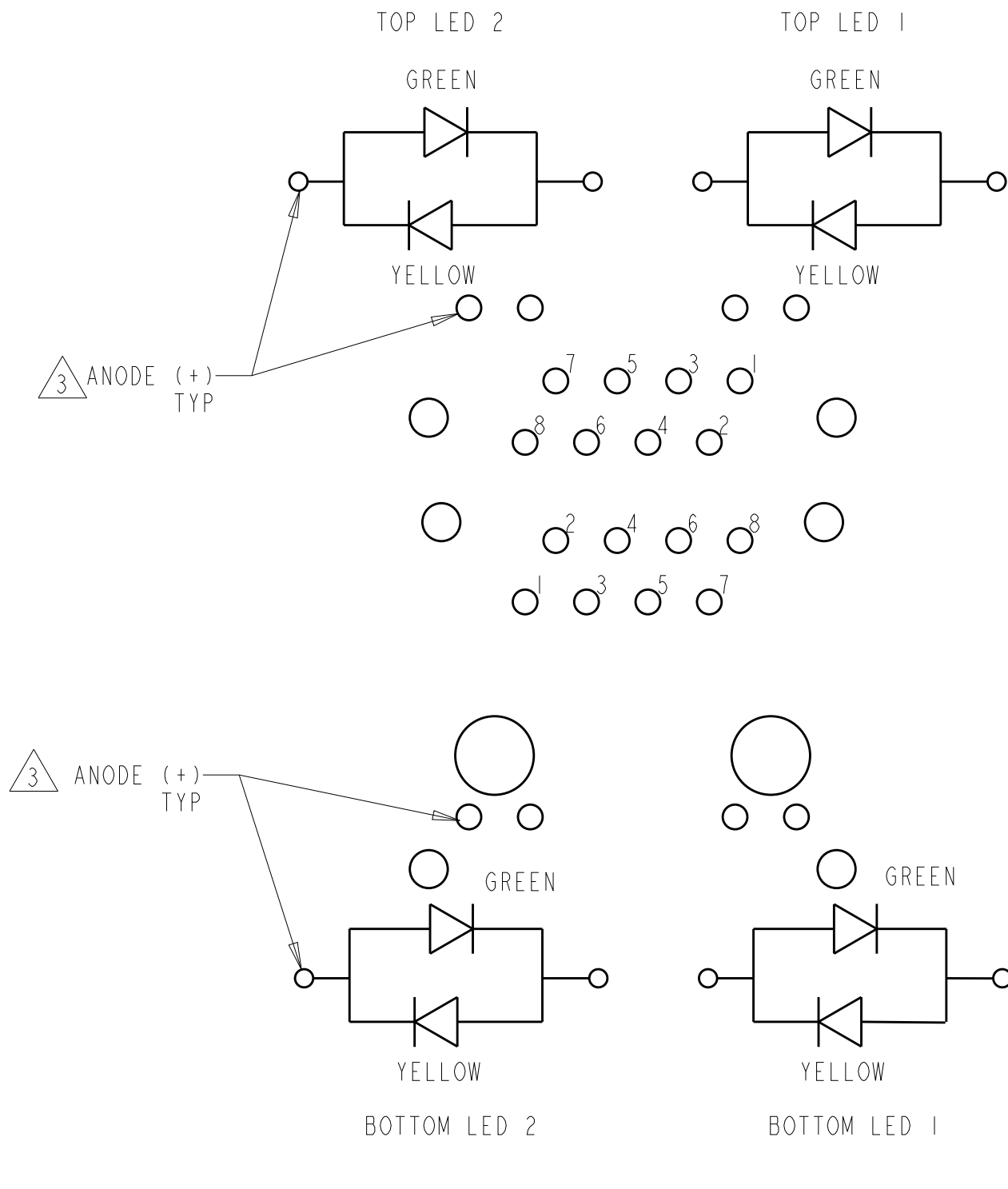
SCHEMATIC FOR 1-6368011-1 SCALE 4:1
