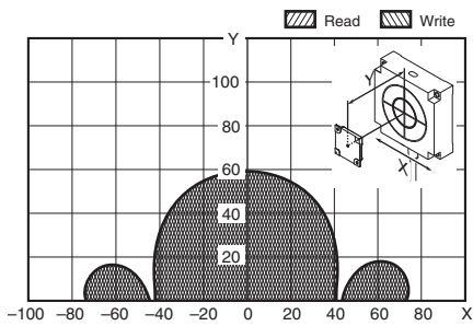
V680-HS63 (with Metal on Back Surface) & V680S-D2KF68 (Tag direction: Horizontal)
