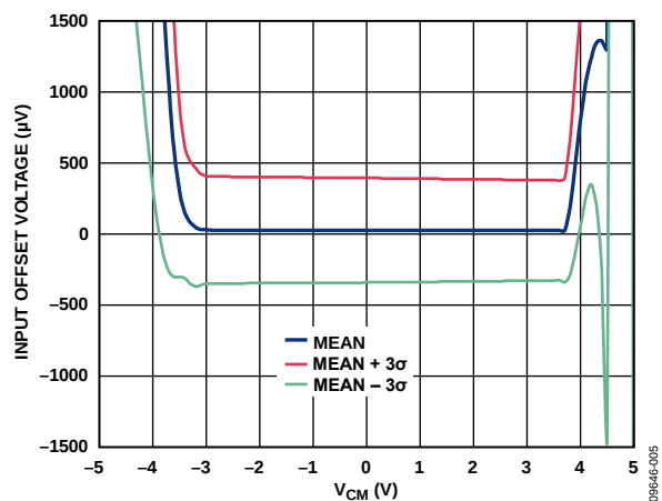
Figure 10. Input Offset Voltage vs. Common-Mode Input Voltage ( V_{CM} ), V_{SV} = \pm 5\text{ V} , R_L = \infty
