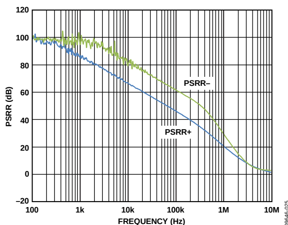
Figure 31. PSRR vs. Frequency, V_{SV} = \pm 15 V
