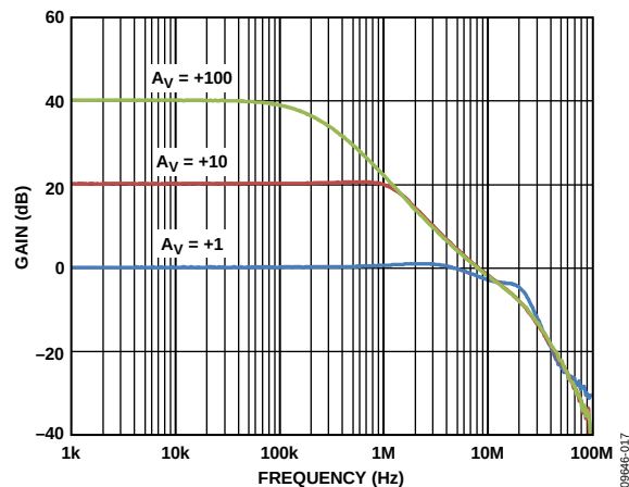
Figure 26. Closed-Loop Gain vs. Frequency, V_{SV} = \pm 5 V
