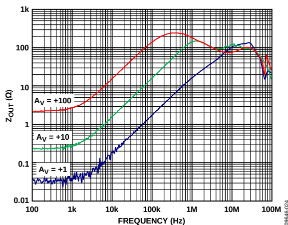
Figure 30. Closed-Loop Output Impedance ( Z_{OUT} ) vs. Frequency, V_{SV} = \pm 15 V
