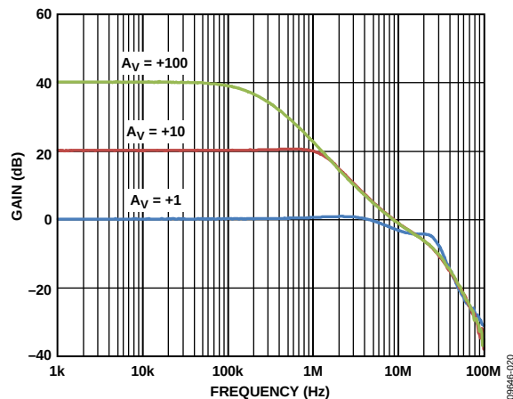
Figure 29. Closed-Loop Gain vs. Frequency, V_{SV} = \pm 15 V
