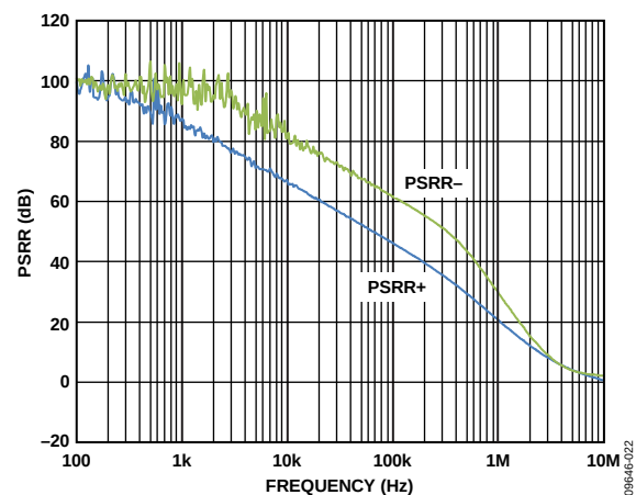
Figure 28. PSRR vs. Frequency, V_{SV} = \pm 5 V
