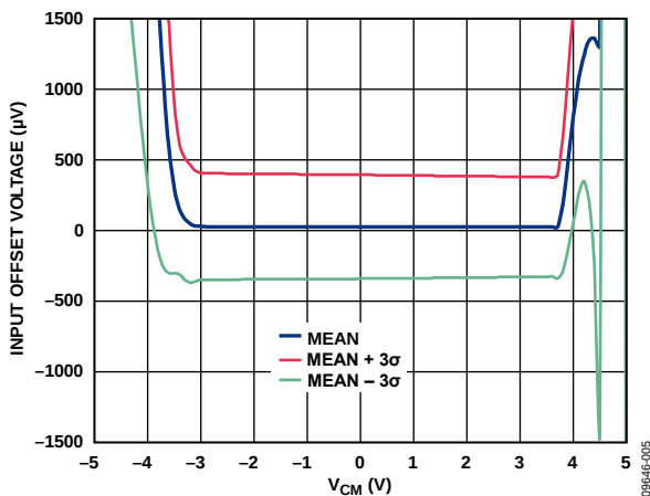
Figure 10. Input Offset Voltage vs. Common-Mode Input Voltage ( V_{CM} ), V_{SY} = \pm 5\text{ V} , R_L = \infty
