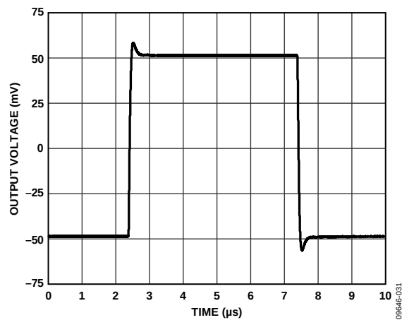
Figure 37. Small Signal Transient Response, V_{SV} = \pm 15\text{ V} , A_V = +1 , R_L = 2\text{ k}\Omega , C_L = 100\text{ pF}
