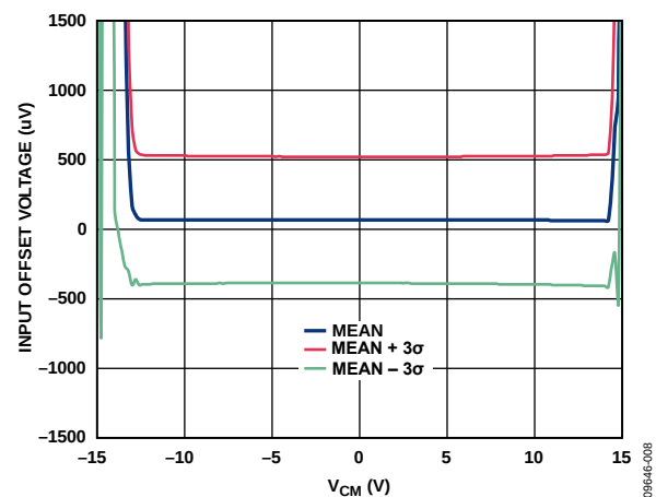
Figure 13. Input Offset Voltage vs. Input Common-Mode Voltage ( V_{CM} ), V_{SY} = \pm 15\text{ V} , R_L = \infty
