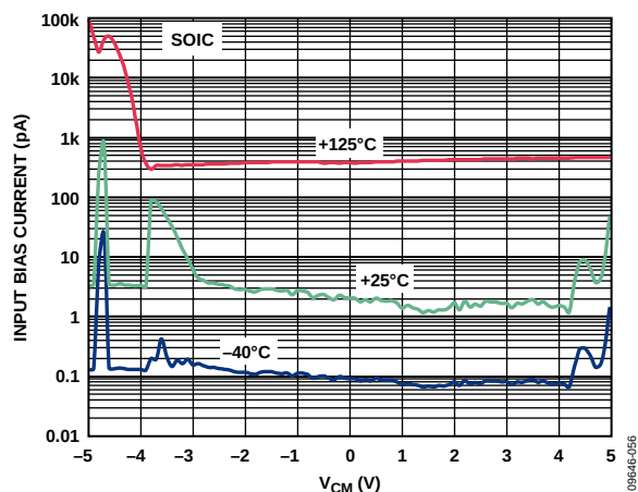
Figure 15. Input Bias Current vs. Common-Mode Input Voltage ( V_{CM} ), V_{SV} = \pm 5\text{ V} , R_L = \infty
