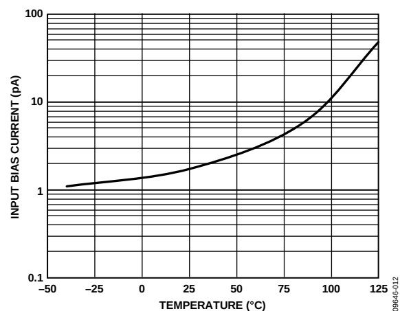
Figure 19. Input Bias Current vs. Temperature, V_{SV} = \pm 15\text{ V}
