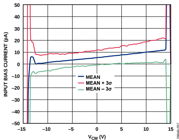
Figure 17. Input Bias Current vs. Common-Mode Input Voltage ( V_{CM} ), V_{SV} = \pm 15\text{ V} , R_L = \infty
