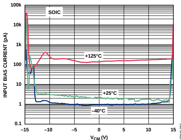
Figure 18. Input Bias Current vs. Common-Mode Input Voltage ( V_{CM} ), V_{SV} = \pm 15\text{ V} , R_L = \infty
