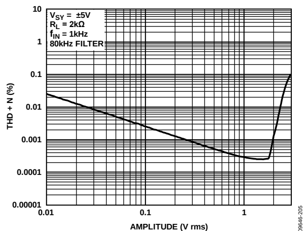
Figure 42. THD + N vs. Amplitude, V_{SY} = \pm 5\text{ V}
