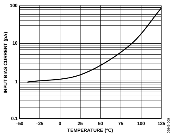
Figure 16. Input Bias Current vs. Temperature, V_{SV} = \pm 5\text{ V}
