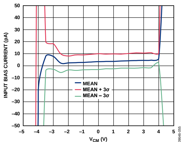
Figure 14. Input Bias Current vs. Common-Mode Input Voltage ( V_{CM} ), V_{SV} = \pm 5\text{ V} , R_L = \infty
