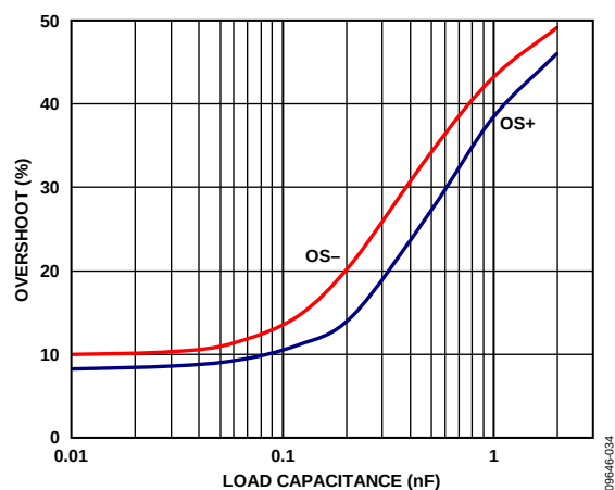
Figure 39. Overshoot vs. Load Capacitance, V_{SY} = \pm 5\text{ V} , A_V = +1 , R_L = 2\text{ k}\Omega , V_{IN} = 100\text{ mV p-p}
