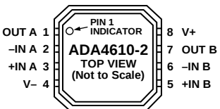
Figure 5. ADA4610-2 Pin Configuration, 8-Lead LFCSP_VD (CP Suffix)
