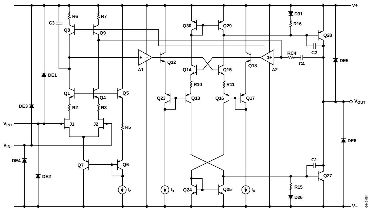
Figure 56. Simplified Schematic
