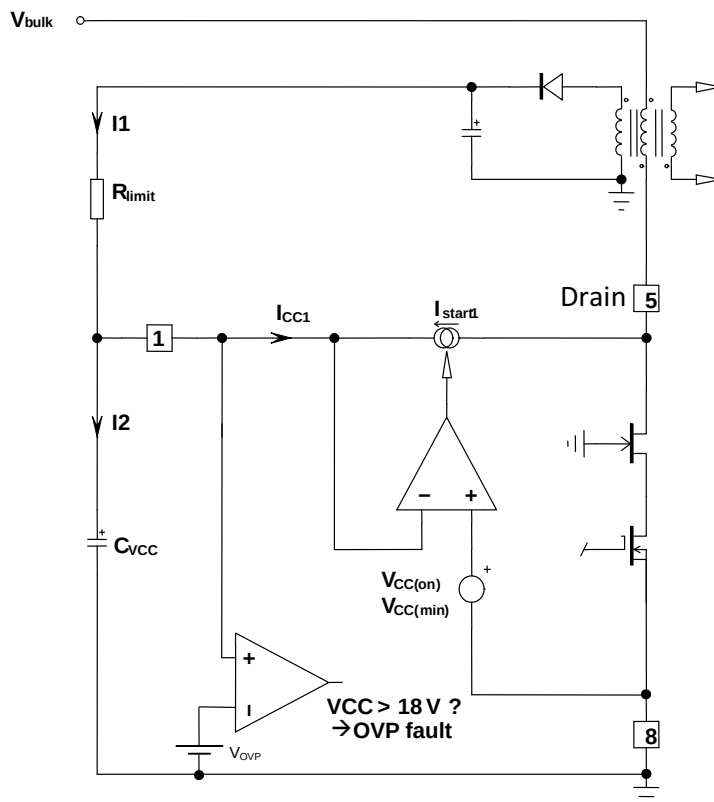
Being loaded by the circuit consumption, the voltage on the V_{CC} capacitor goes down. When V_{CC} is below V_{CC(min)} level (7.5 V typically), it activates the internal current source to bring V_{CC} toward V_{CC(on)} level and stops again: a cycle takes place whose low frequency depends on the V_{CC}
