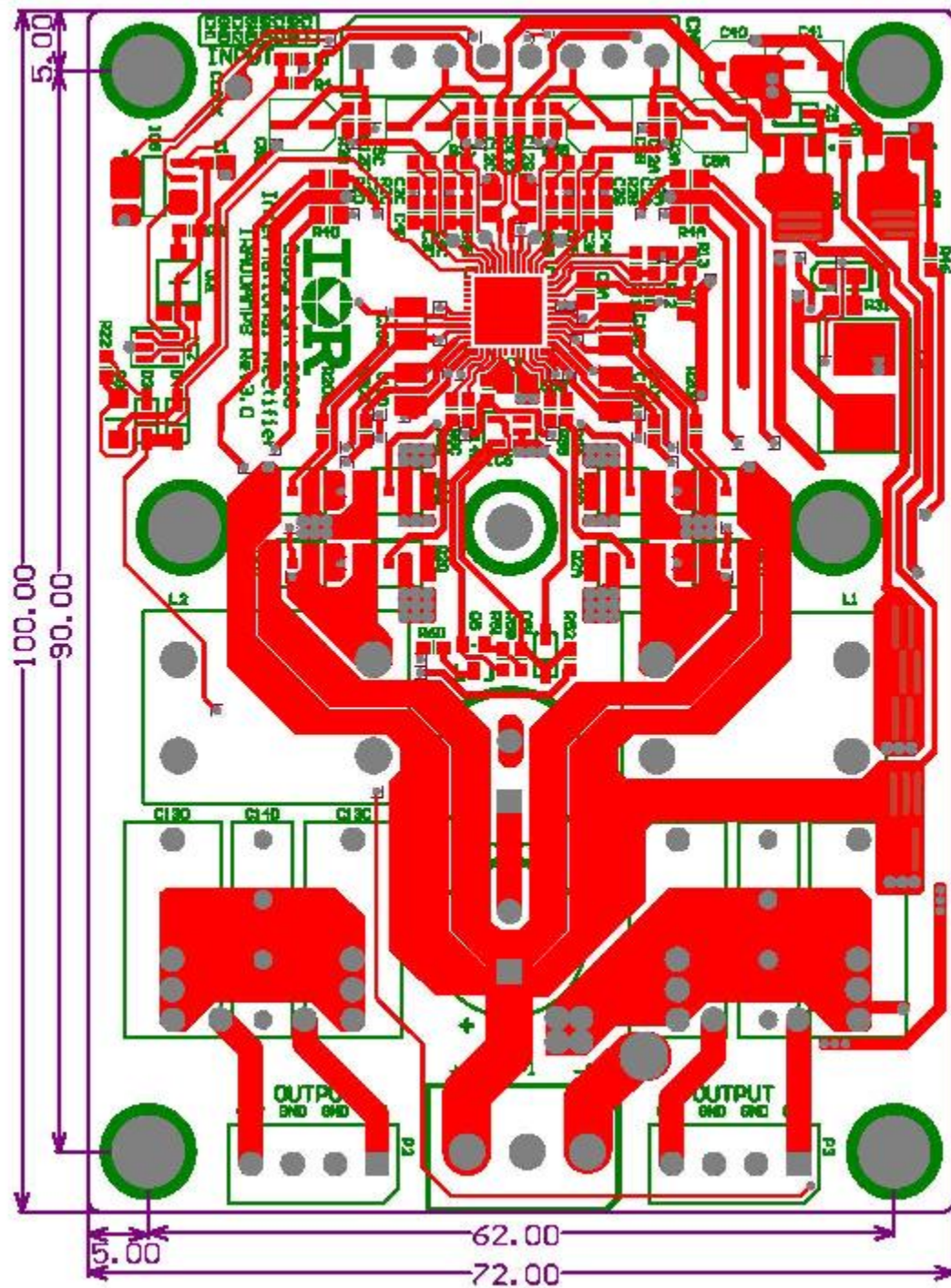
Fig 25 IRAUDAMP8 PCB Top Overlay (Top View)
