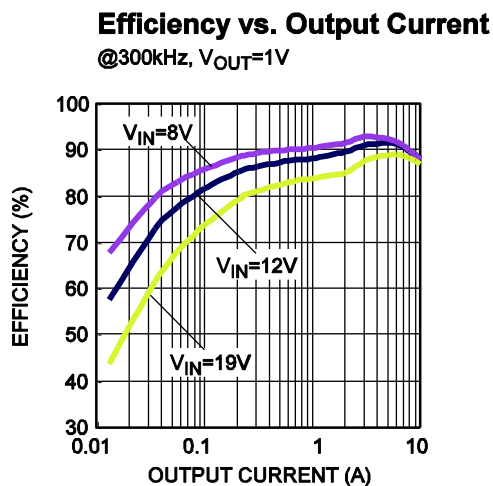
Figure 18 — Efficiency Curve
