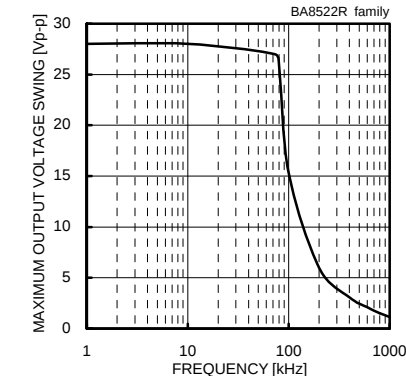
Fig. 197 Maximum Output Voltage Swing - Frequency ( V_{CC}/V_{EE}=+15[V]/-15[V] , R_L=2[k\Omega] , T_a=25[^\circ C] )
