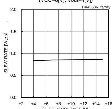
Slew Rate - Supply Voltage ( C_L=100[pF] , R_L=2[k\Omega] , T_a=25[°C] )
