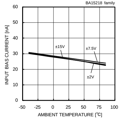
Input Bias Current - Ambient Temperature (V icm =0[V], V out =0[V])
