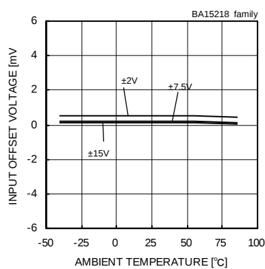
Input Offset Voltage - Ambient Temperature (V icm =0[V], V out =0[V])
