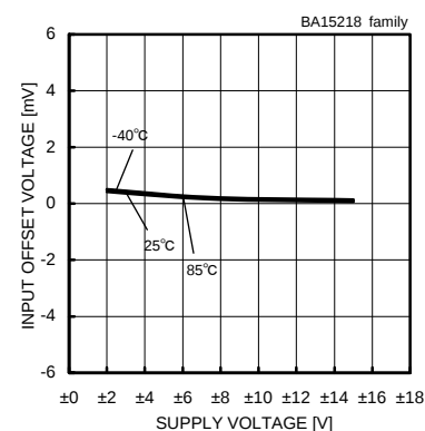
Input Offset Voltage - Supply Voltage (V icm =0[V], V out =0[V])
