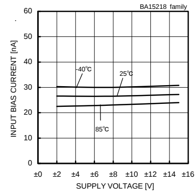
Input Bias Current - Supply Voltage (V icm =0[V], V out =0[V])
