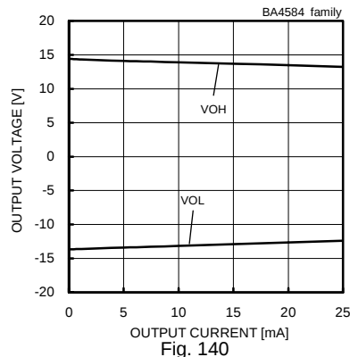
Fig. 140 Maximum Output Voltage - Output Current (VCC/VEE=+15[V]/-15[V], Ta=25[°C])
