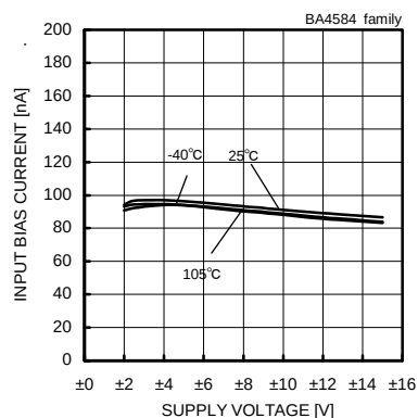
Fig. 143 Input Bias Current - Supply Voltage (Vcm=0[V], Vout=0[V])
