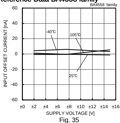
Input Offset Current - Supply Voltage ( V_{icm}=0[V] , V_{out}=0[V] )
