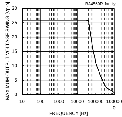
Fig. 87 Maximum Output Voltage Swing - Frequency ( V_{CC}/V_{EE}=+15[V]/-15[V] , R_L=2[k\Omega] , T_a=25[°C] )
