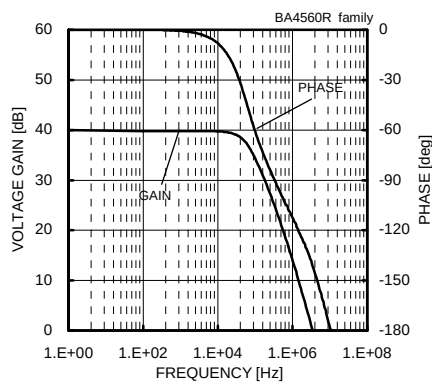
Fig. 88 Voltage Gain - Frequency ( V_{CC}/V_{EE}=+15[V]/-15[V] , A_v=40[dB] , R_L=2[k\Omega] , T_a=25[°C] )
