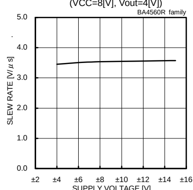
Fig. 84 Slew Rate - Supply Voltage ( C_L=100[pF] , R_L=2[k\Omega] , T_a=25[°C] )
