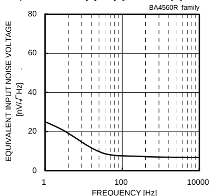
Fig. 85 Equivalent Input Noise Voltage - Frequency ( V_{CC}/V_{EE}=+15[V]/-15[V] , R_s=100[\Omega] , T_a=25[°C] )
