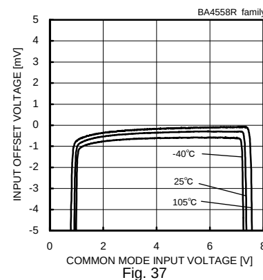
Input Offset Voltage - Common Mode Input Voltage ( V_{CC}=8[V] , V_{out}=4[V] )
