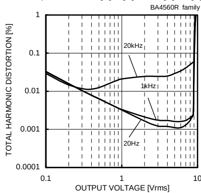
Fig. 86 Total Harmonic Distortion - Output Voltage ( V_{CC}/V_{EE}=+15[V]/-15[V] , A_v=20[dB] , R_L=2[k\Omega] , 80[kHz] -LPF, T_a=25[°C] )
