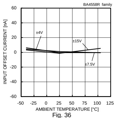
Input Offset Current - Ambient Temperature ( V_{icm}=0[V] , V_{out}=0[V] )
