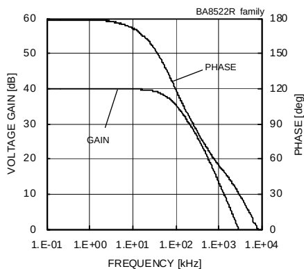
Fig. 198 Voltage Gain - Frequency ( V_{CC}/V_{EE}=+15[V]/-15[V] , A_v=40[dB] , R_L=2[k\Omega] , T_a=25[^\circ C] )
