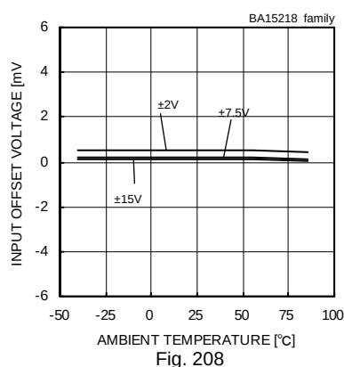
Input Offset Voltage - Ambient Temperature (Vicm=0[V], Vout=0[V])
